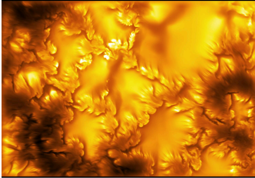
The highest-resolution image of the sun's surface ever captured NSF / NSO / AURA / MPS
